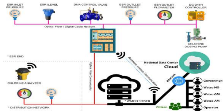
Figure 8: System Architecture of Smart Water Management System In Puri
