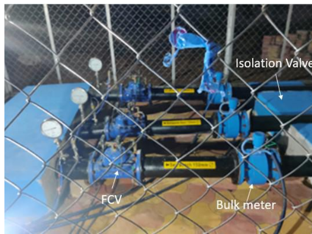
Figure 6: Outlet arrangement of ESR
